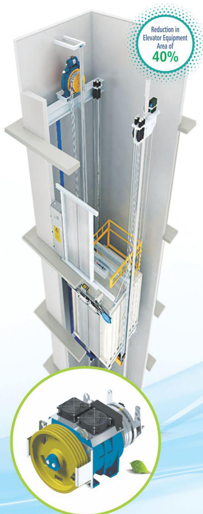
Gearless Machine
