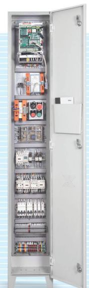
STEP Elevator Serial Integrated Controller
